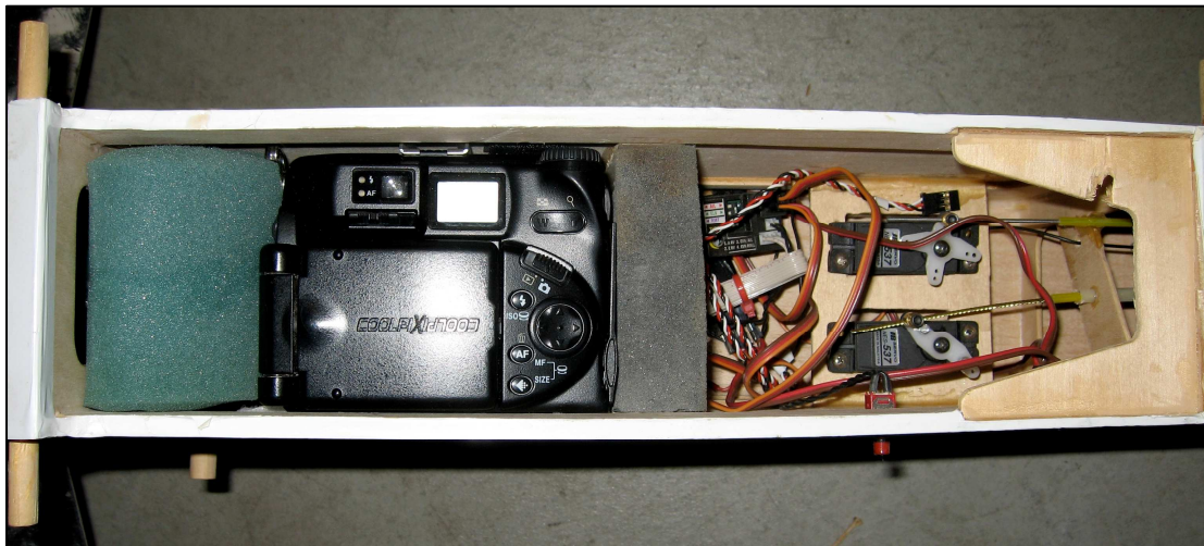
The camera inside the aircraft.. The DigiSnap was located under the nose hatch and the Gecko was secured on top of the nose hatch by Velcro and a rubber band.
